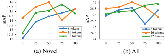
Figure 4: Effectiveness of tokens of vision-guided language prompts on the VidVRD dataset. The x-axis represents the percentage of tokens from conditional prompts, from 0 (all tokens are from learnable continuous prompts) to 100% (all tokens are from learnable conditional prompts), and different colors denote different lengths.
